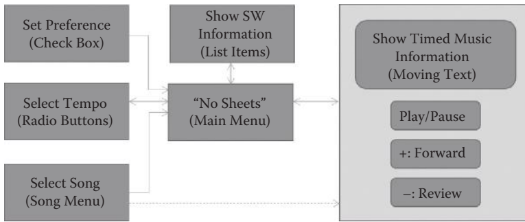
Figure 4.20 A possible state-transition diagram for No Sheets.
