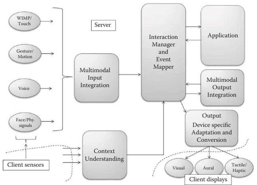
Figure 9.21 Middleware architecture for supporting the cloud–client application platform.
